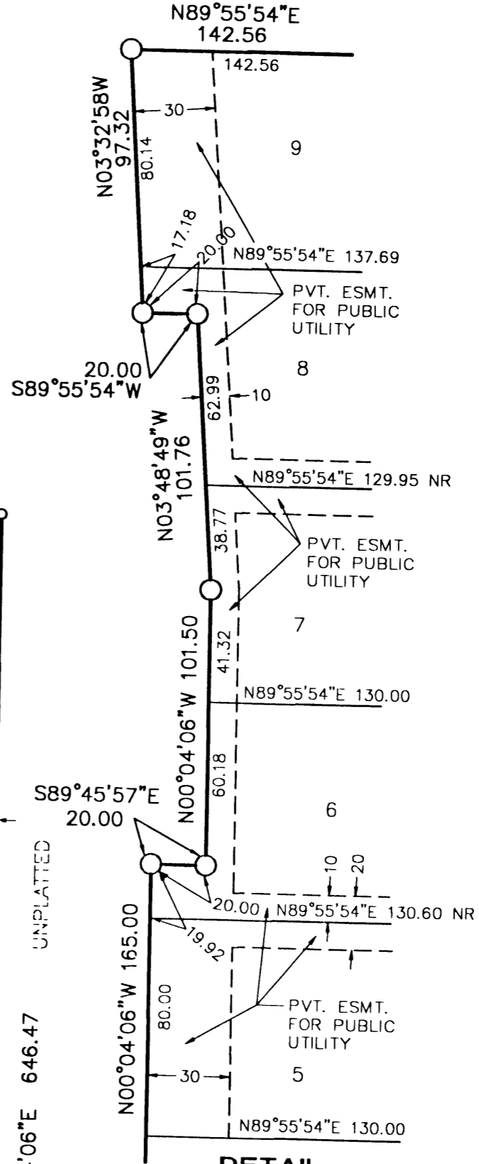
DETAIL 1"=50'
