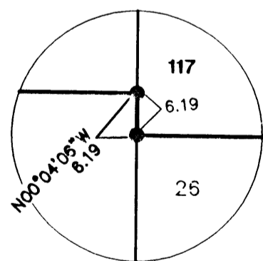
DETAIL 1"=20'
